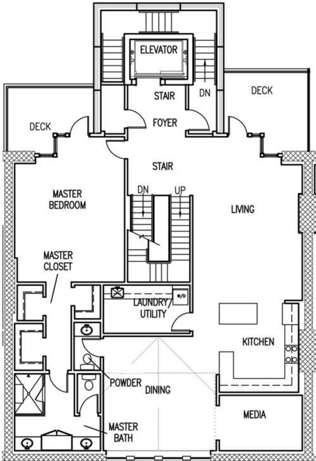
Level One - Third Floor
